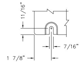
BOLT SLOT DETAIL
